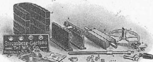
Fig. 15.—Generator Parts.
