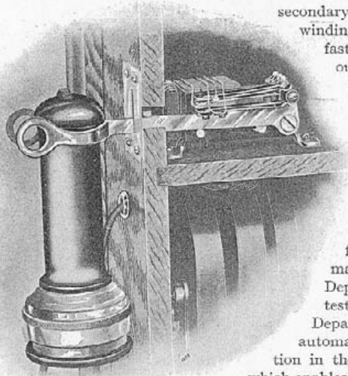
Fig. 10.—Hook-switch.
