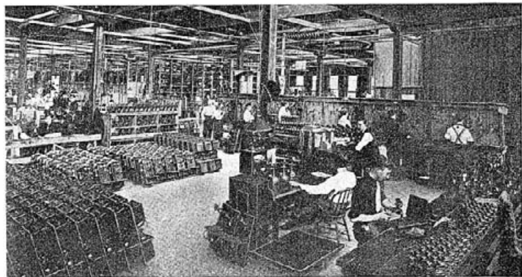
Fig. 13.—Testing Telephones—B.
